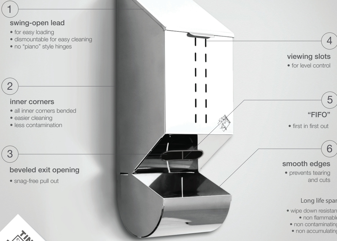
Modular wall / frame mounted dispensers
